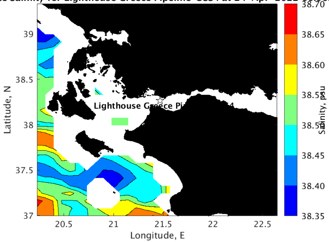
ce Salinity for Lighthouse Greece Pipeline-OSS4 at 24-Apr-2022 00:00:00
